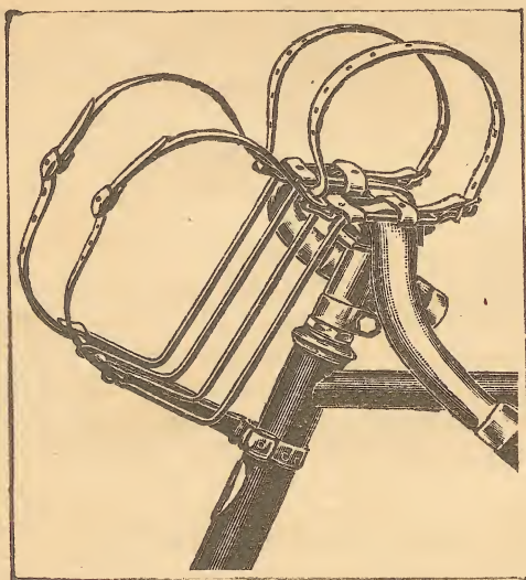
Lamson Double Carrier, No. 4-D. (6 inch drop.)
